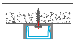
MONTAGGIO A PARETE WALL MOUNTED
