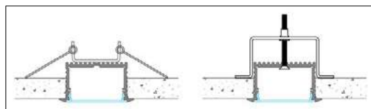
MONTAGGIO A INCASSO FLUSH-MOUNTED
