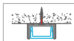
MONTAGGIO A PARETE CON CLIP WALL MOUNTED WITH CLIPS
