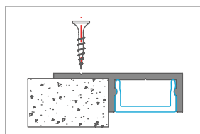
PARETE WALL-MOUNTED
